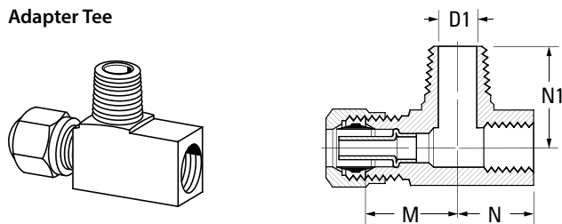
Adapter Tee
