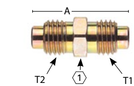
Union Adapter
