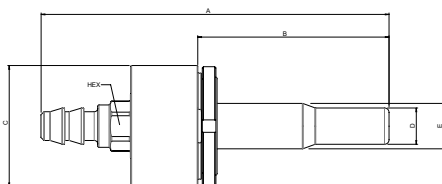
Figure 1 Plug
