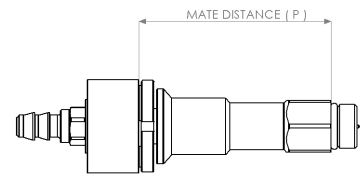
Figure 3 Connected
